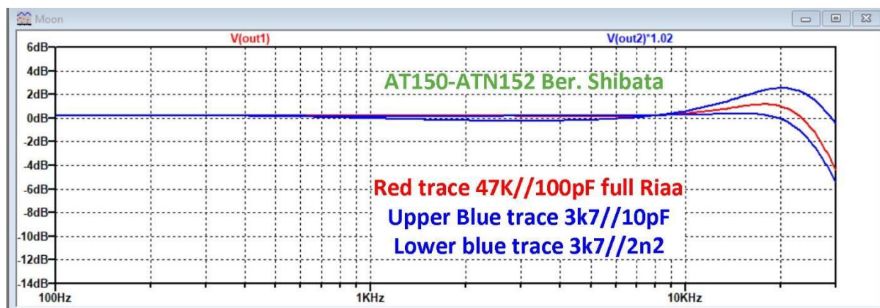
Figure 15, loading the Cart with a 75 \mu sec pole versus 47k//100pF full Riaa
