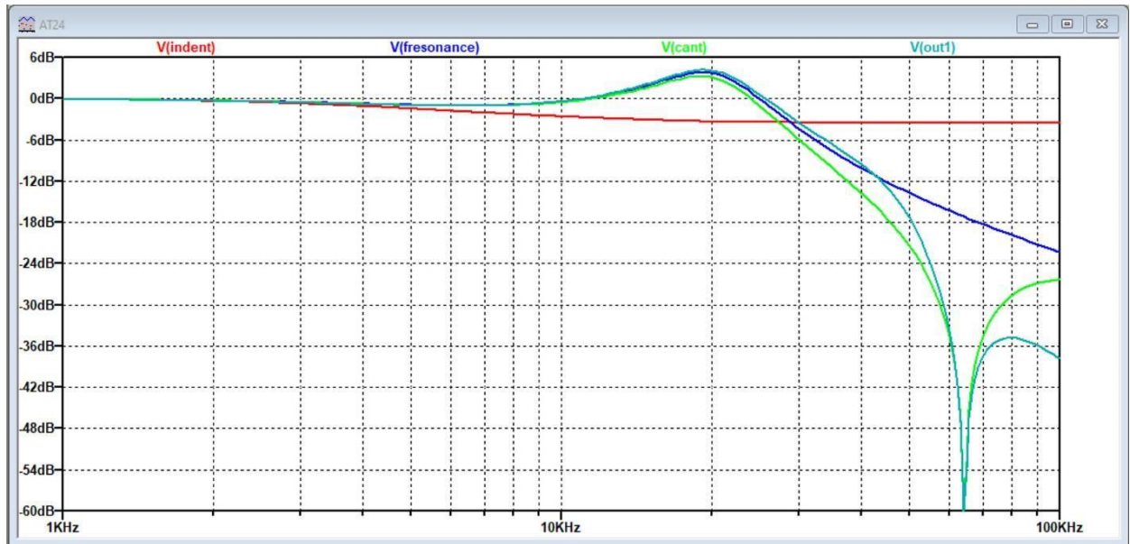
Figure 8, Frequency responses at various point from the AT24-Sapphires Circuit diagram
