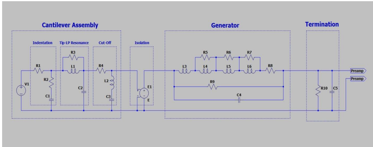
Figure 6, Generic model for Cart plus termination
