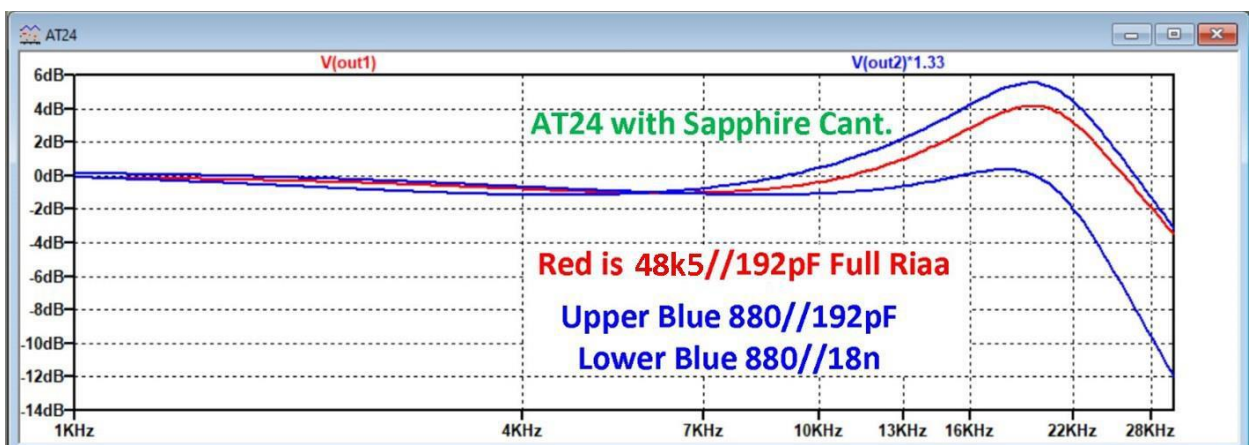
Figure 13, Loading the Cart with a 75\mu\text{sec} pole versus 48K5//192pF full Riaa
