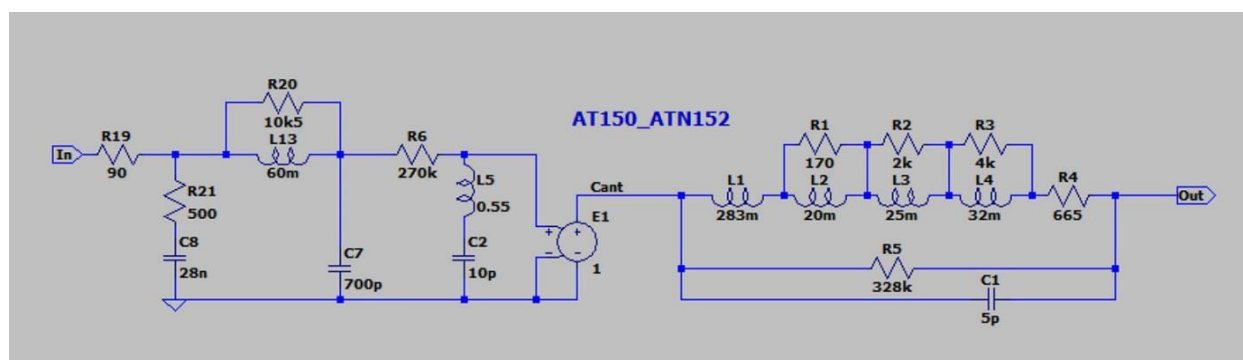
Figure 14, Replacement diagram for the AT150 with 5 \mu m ATN152 Beryllium Shibata tip.
