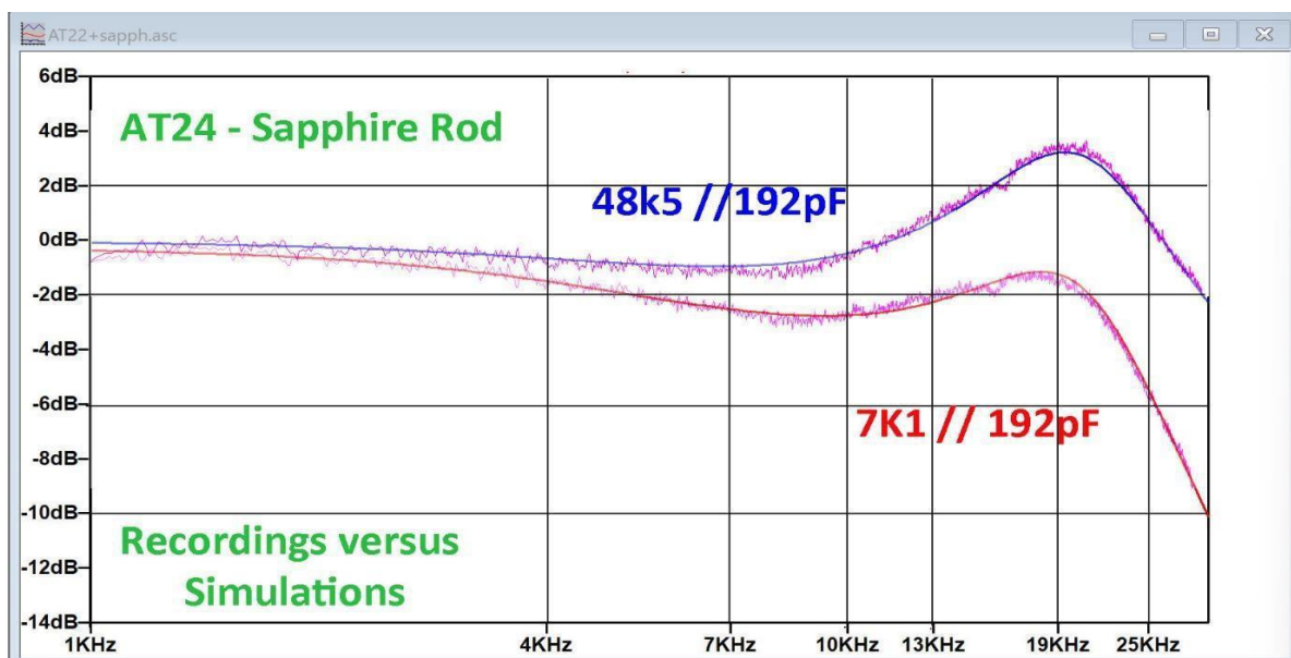
Figure 9, Recorded and simulated FR for two very different load situations
