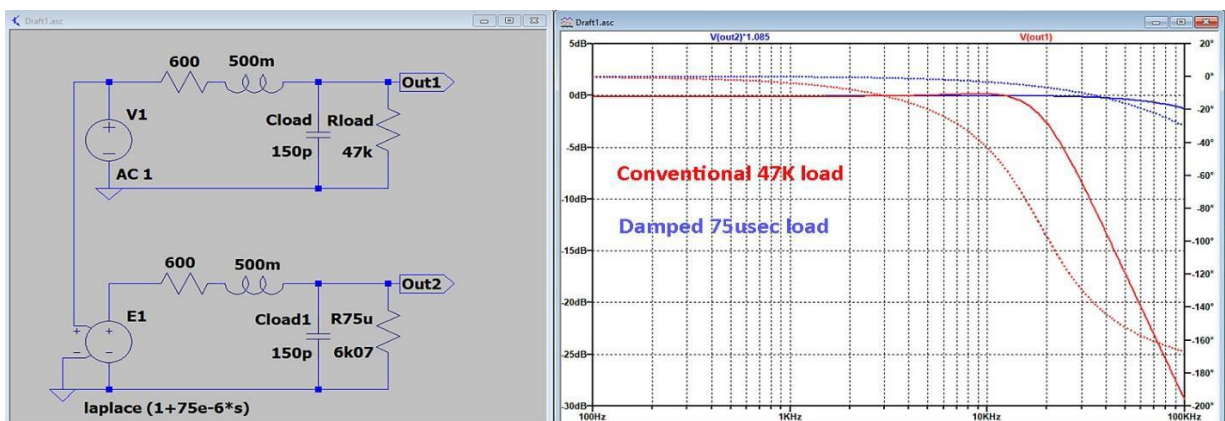
Figure 12, The effect of 75\mu\text{sec} damped loading on a simple Cart model
