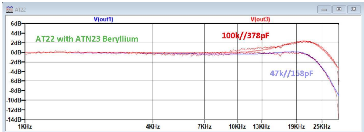
Figure 10, Recording versus simulation for a AT22 with ATN23 Cantilever
