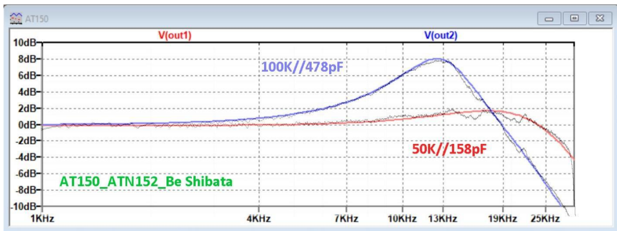
Figure 11, Recording versus simulation for a AT150 with ATN152 Cantilever
