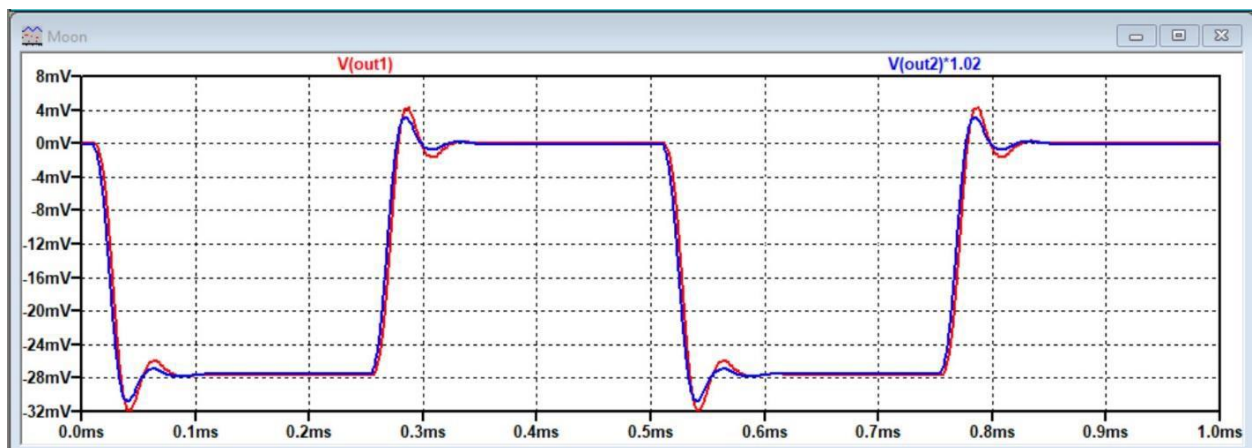
Figure 16, Square wave on AT150_ATN152 with 47k//100p full Riaa and 3K7//2n2 minus T3
