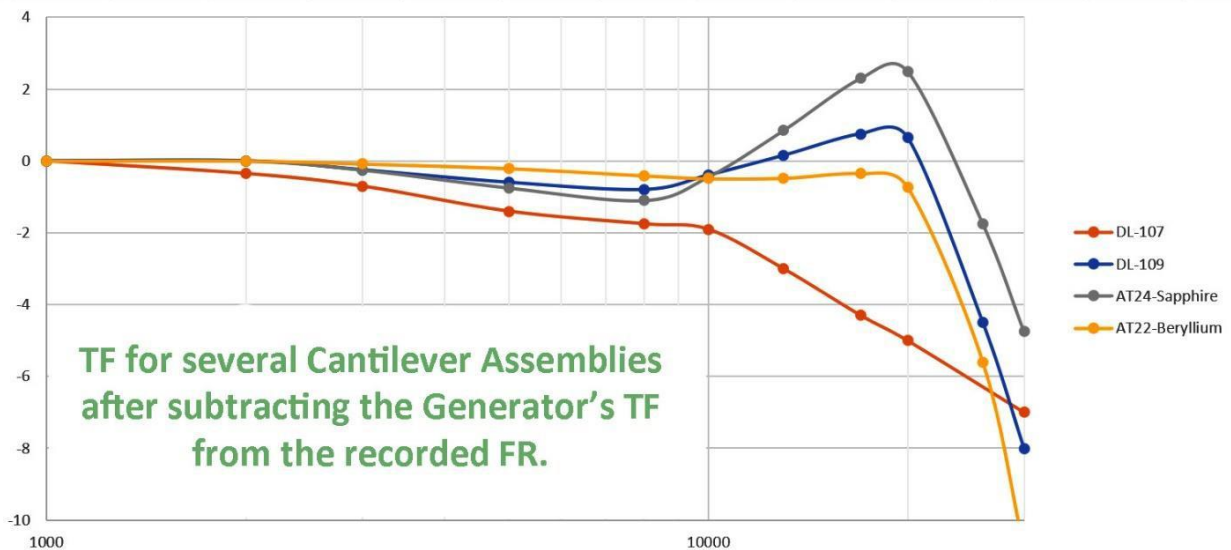
Figure 4, Frequency response for four Cantilever assemblies.
