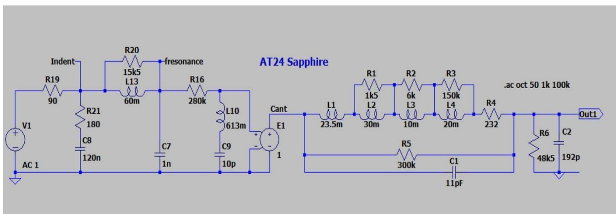
Figure 7, Circuit diagram for a AT24 with Sapphire cantilever and 0.24 mil elliptical tip
