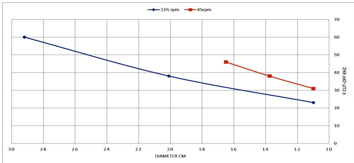
Figure 5, Cut-off frequency dependency on rpm and position for a 0.65 mil round tip.
