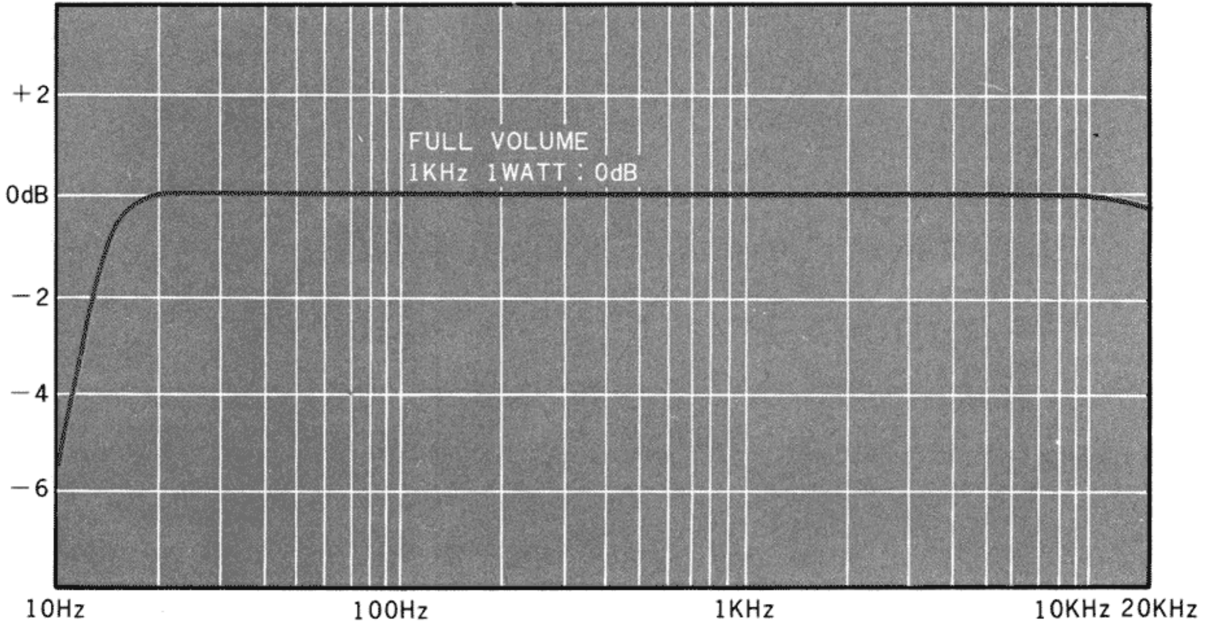
Figure 20. Frequency Response
