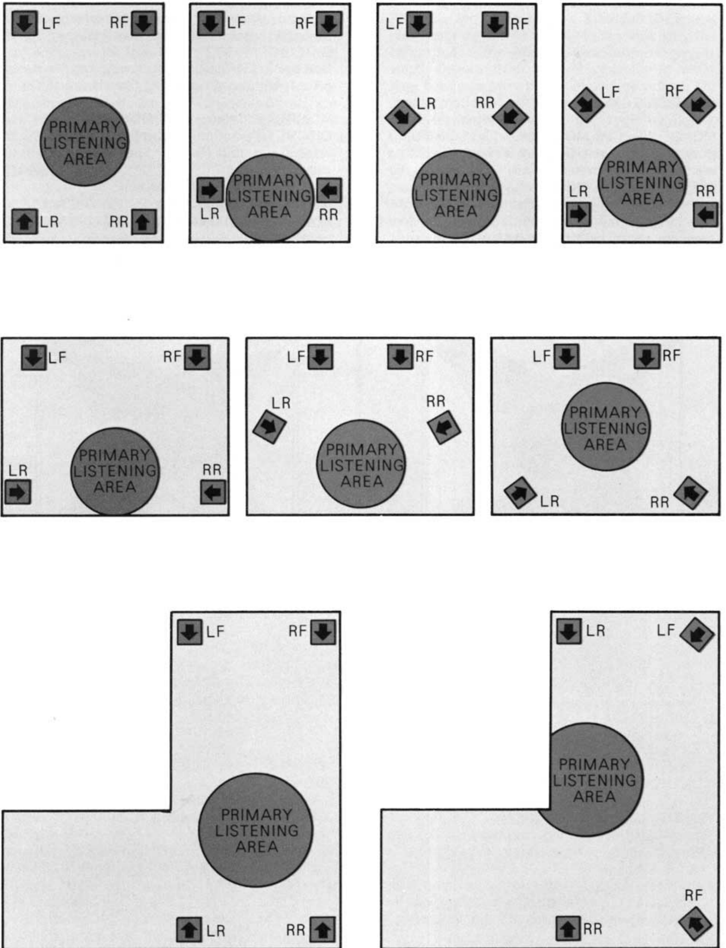
Figure 4. Speaker Placement
