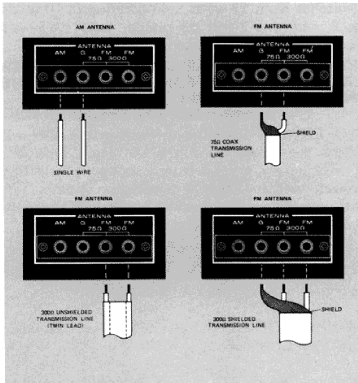
Figure 11. FM/AM Antenna Connections
