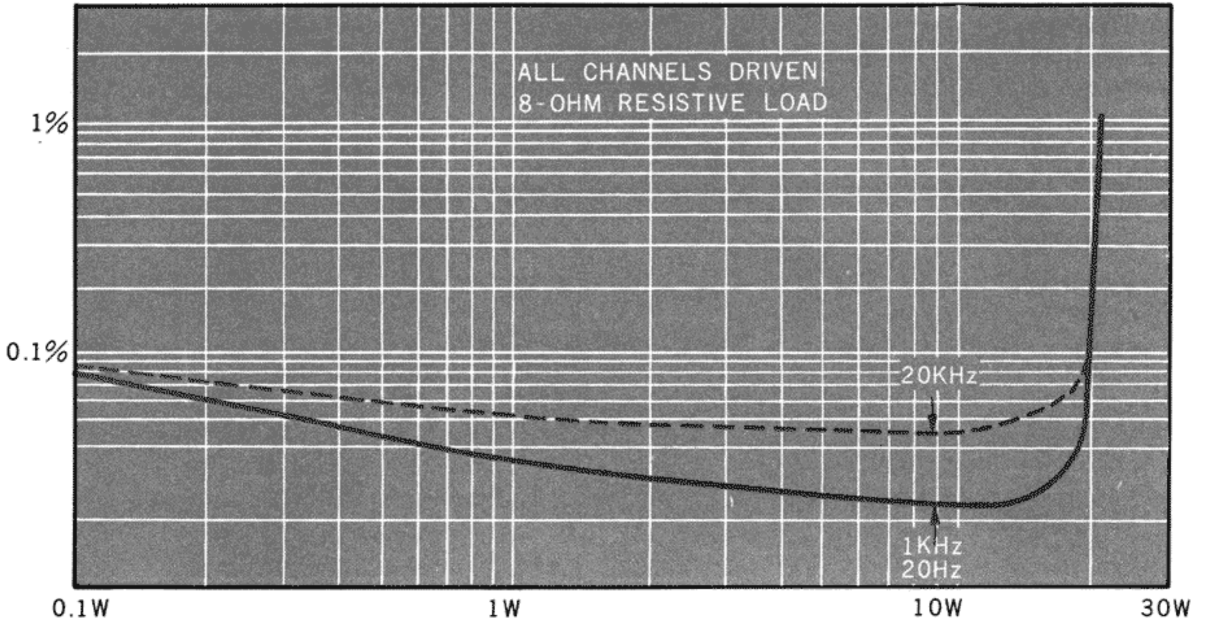
Figure 19. Harmonic Distortion
