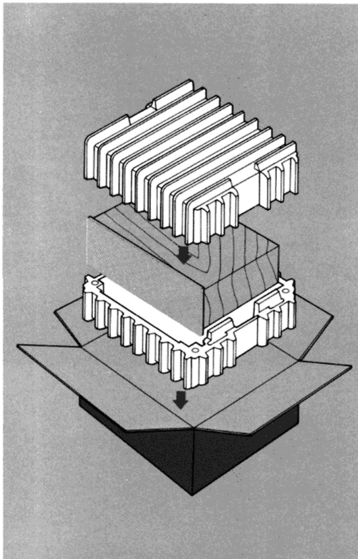
Figure 21. Packing Instructions
