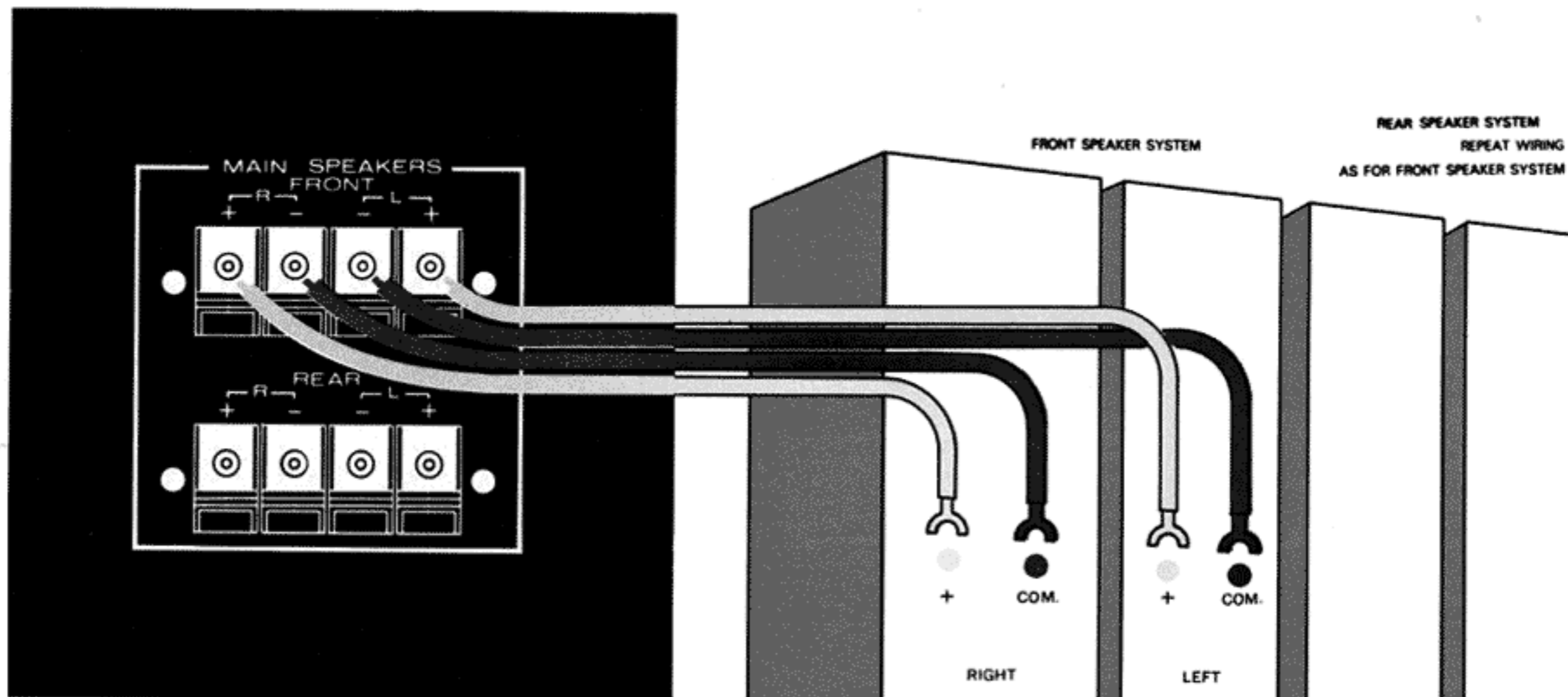
Figure 2. Loudspeaker System Connections
