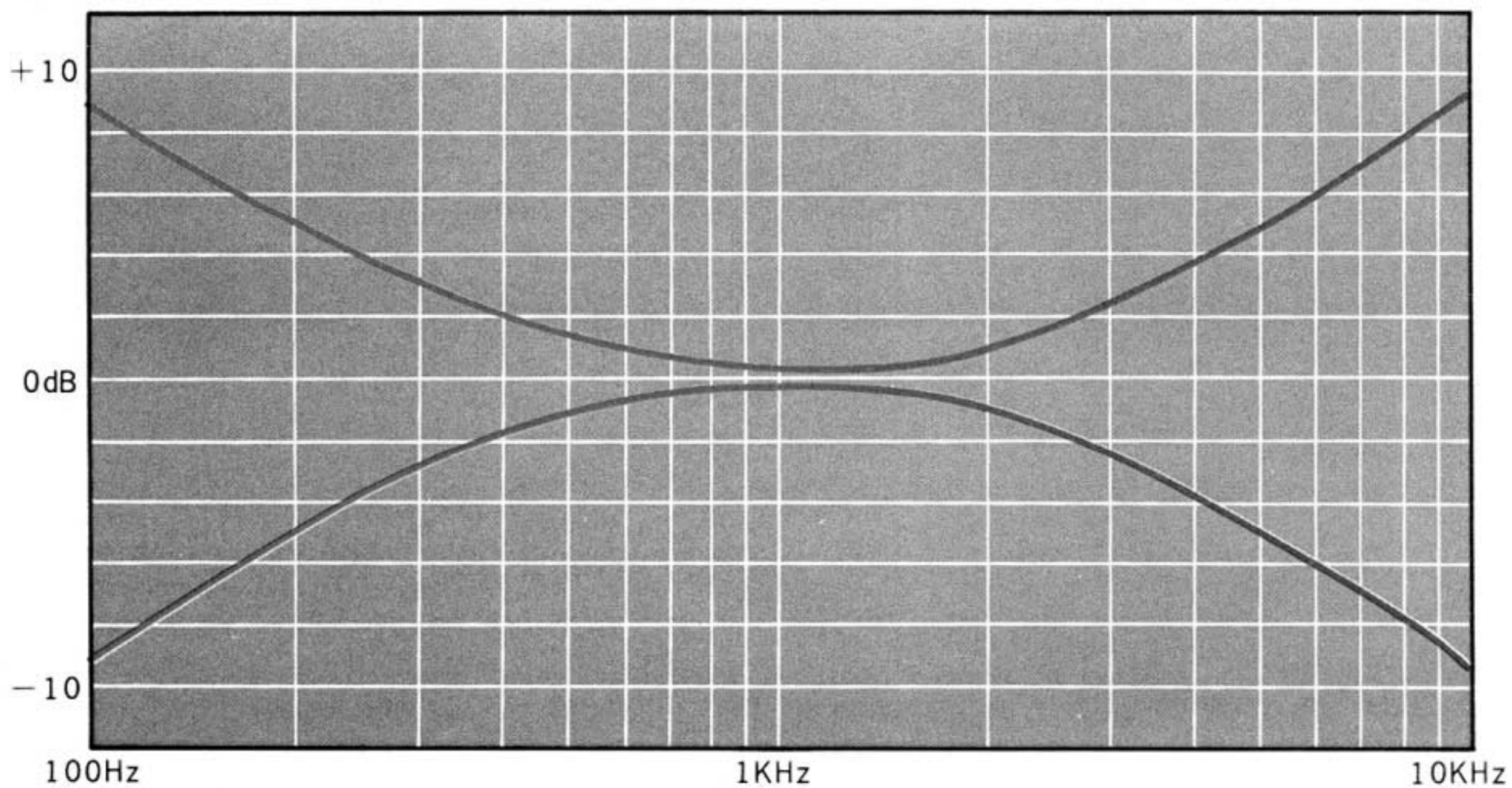
Figure 18. Tone Control Characteristics
