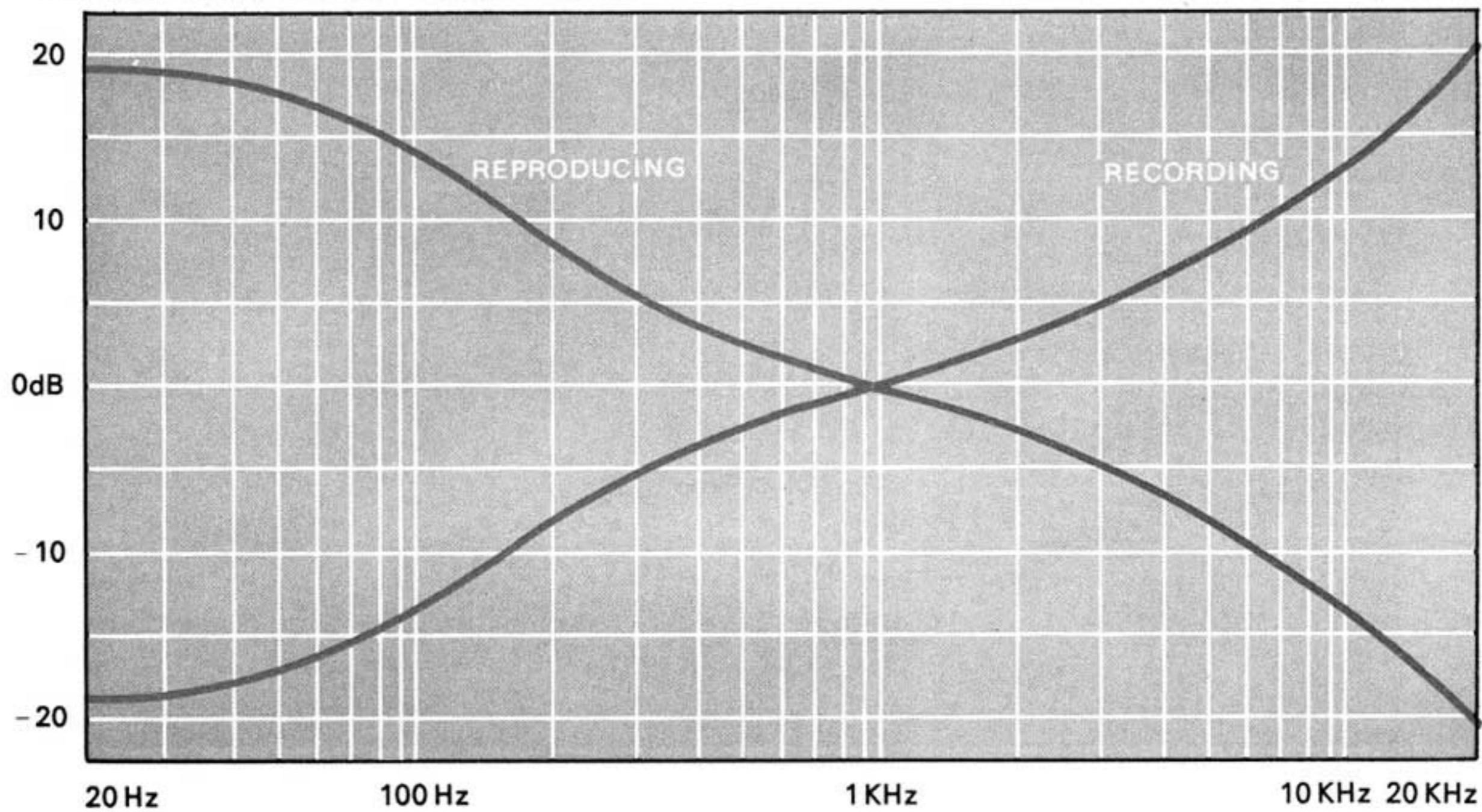
Figure 17. Phono Equalization Characteristics
