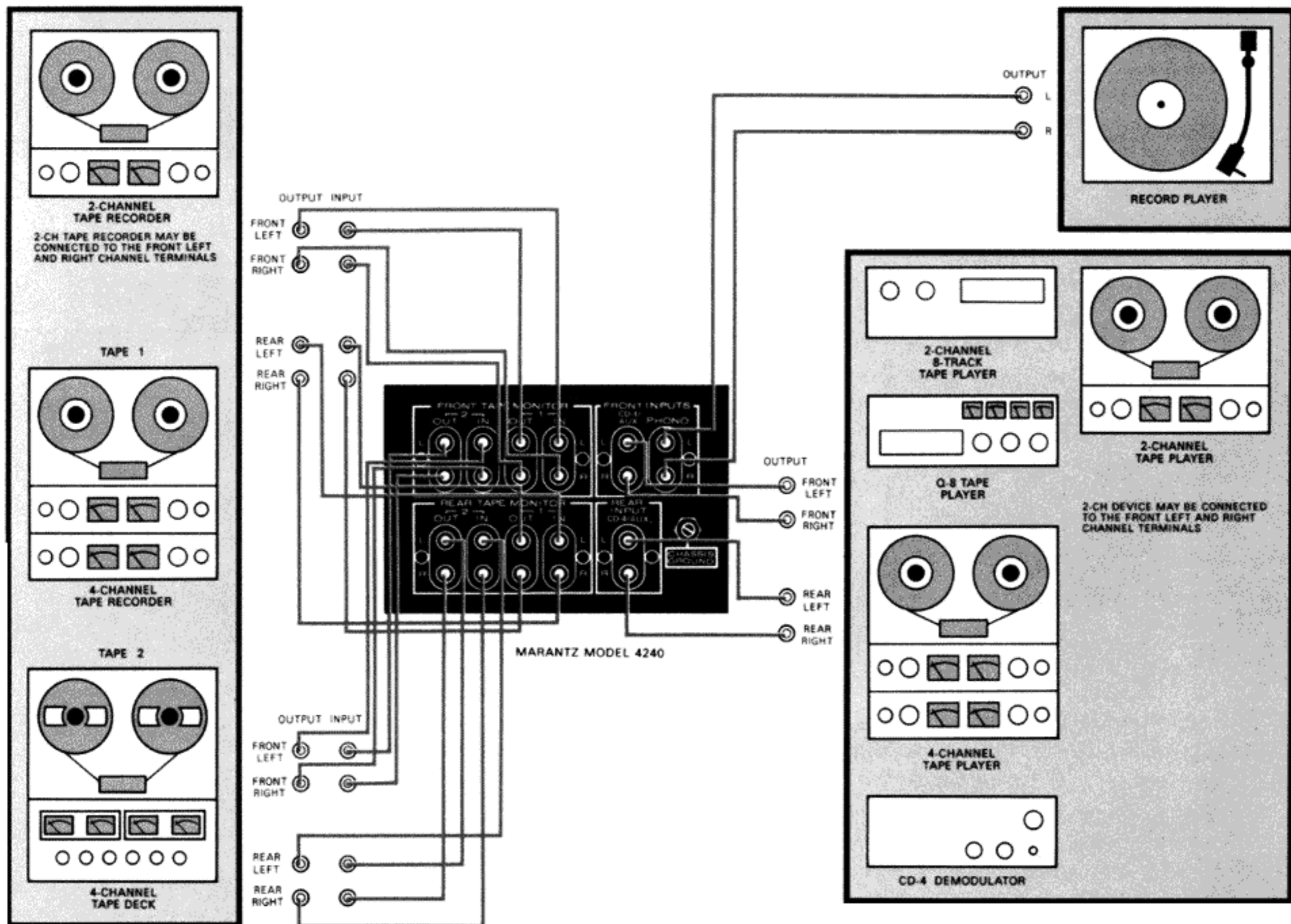
Figure 3. Connection Diagram
