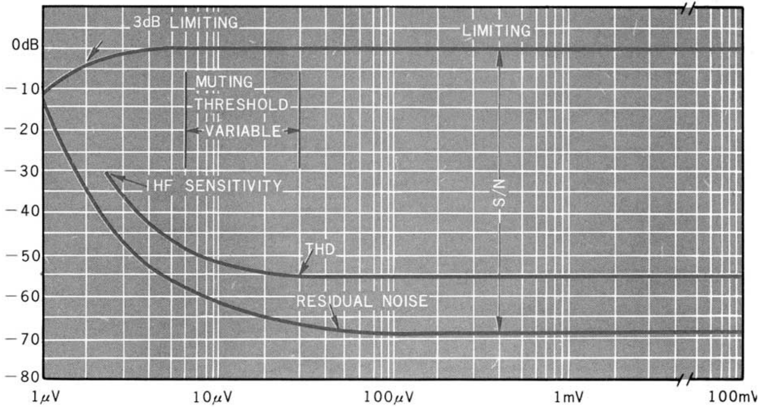
Figure 15. FM Characteristics
