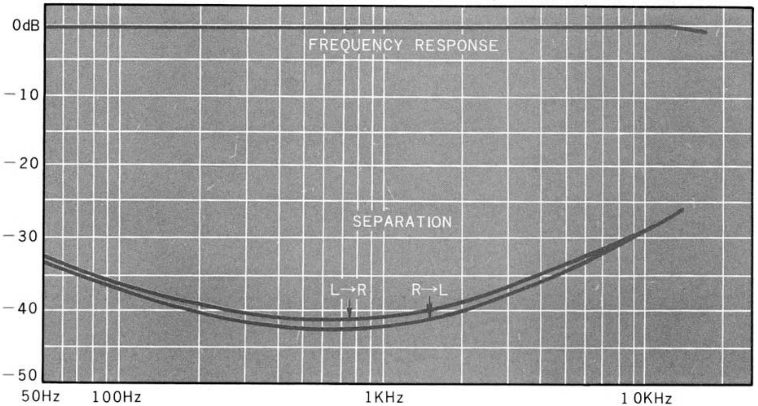
Figure 16. Stereo Separation
