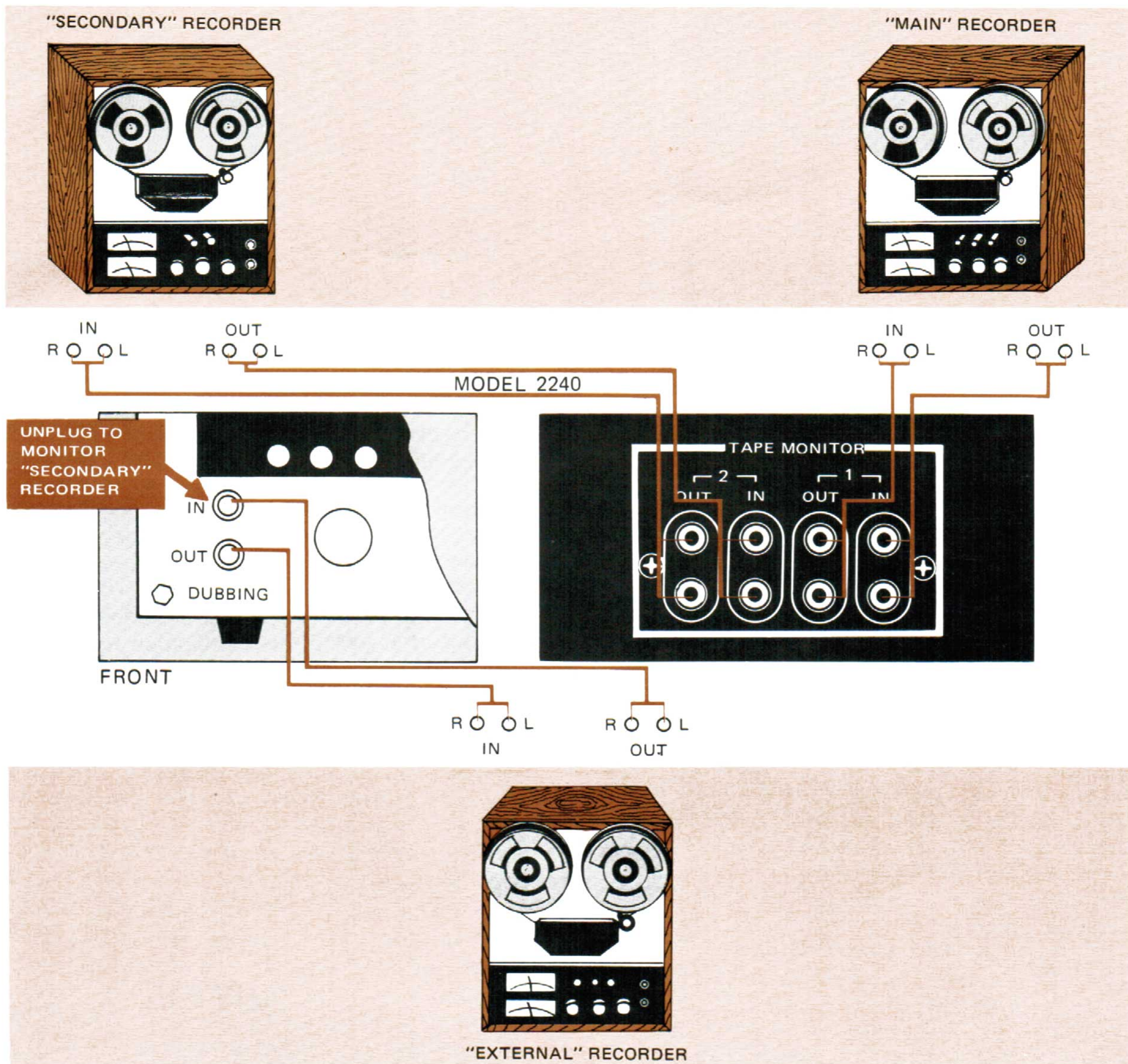
Figure 7. Tape Recorder Connections
