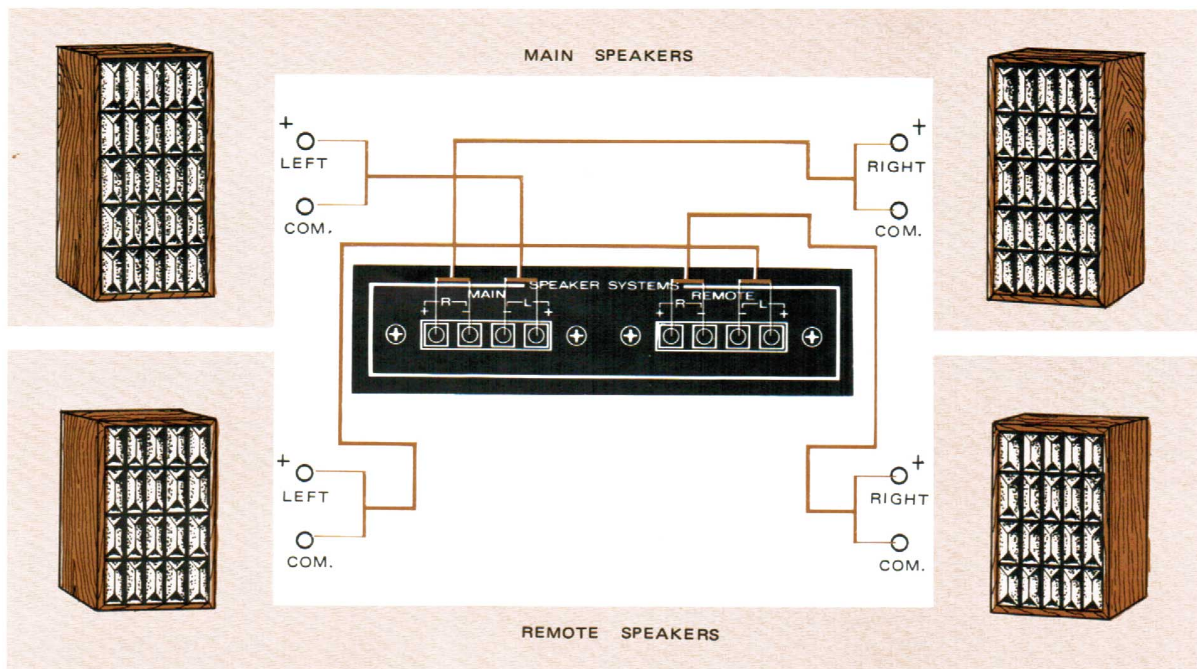
Figure 4. Speaker System Connections
