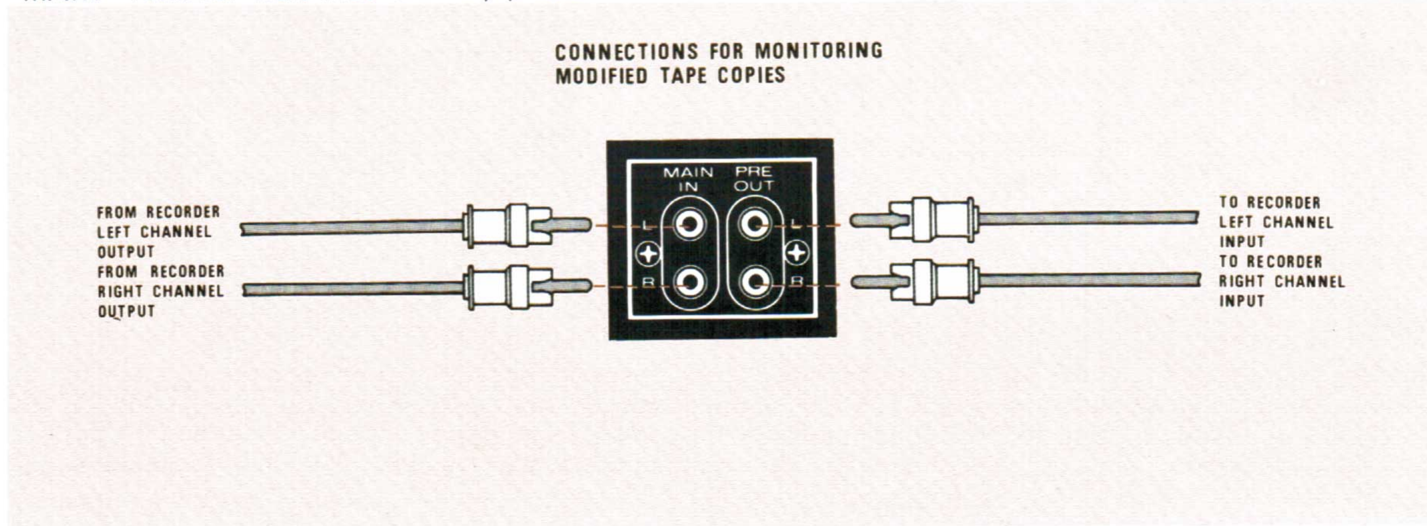
Figure 8. Arrangement for Making Modified Tape Copies
