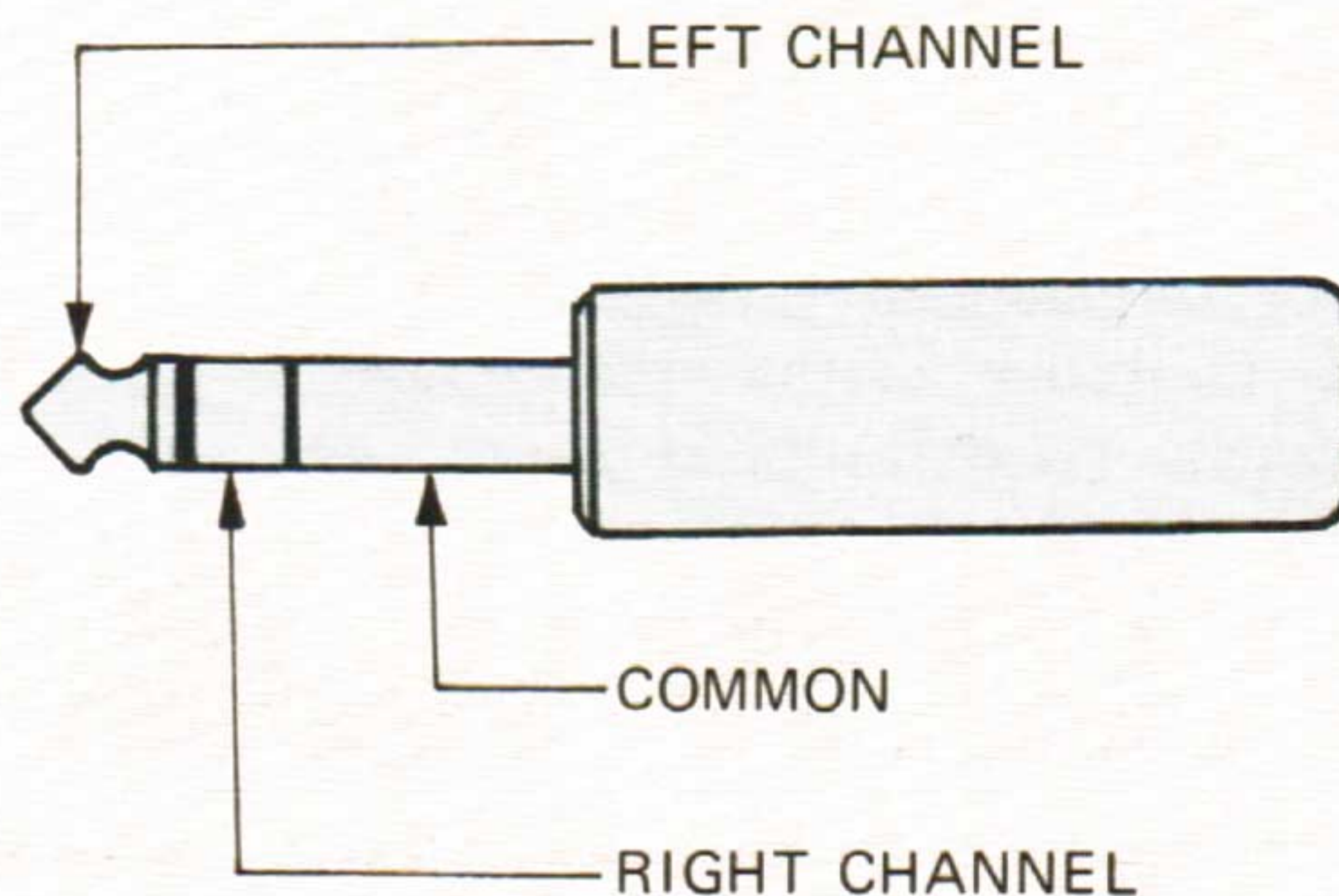
Figure 6. Three Conductor Phone Plug
