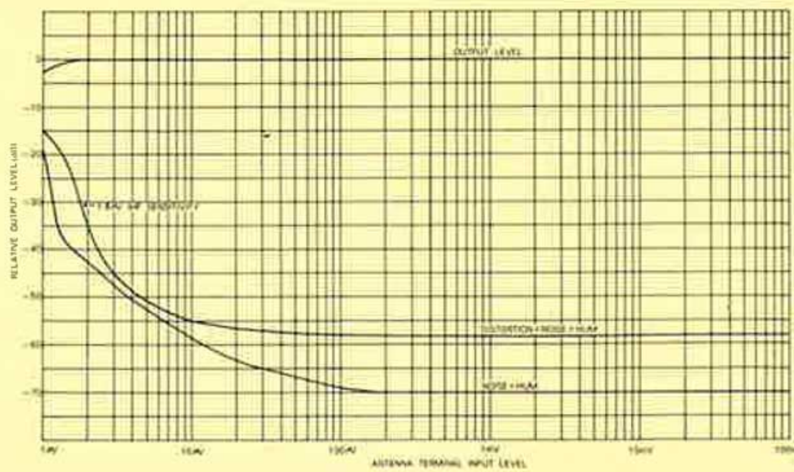
FM CHARACTERISTIC
