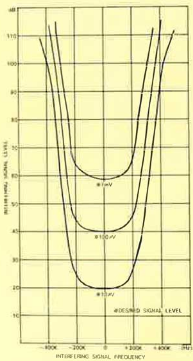
SELECTIVITY
