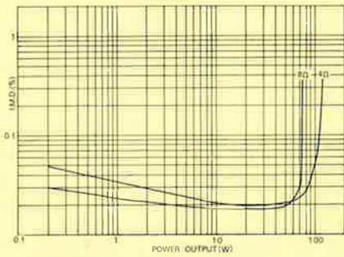
POWER I.M.D.
