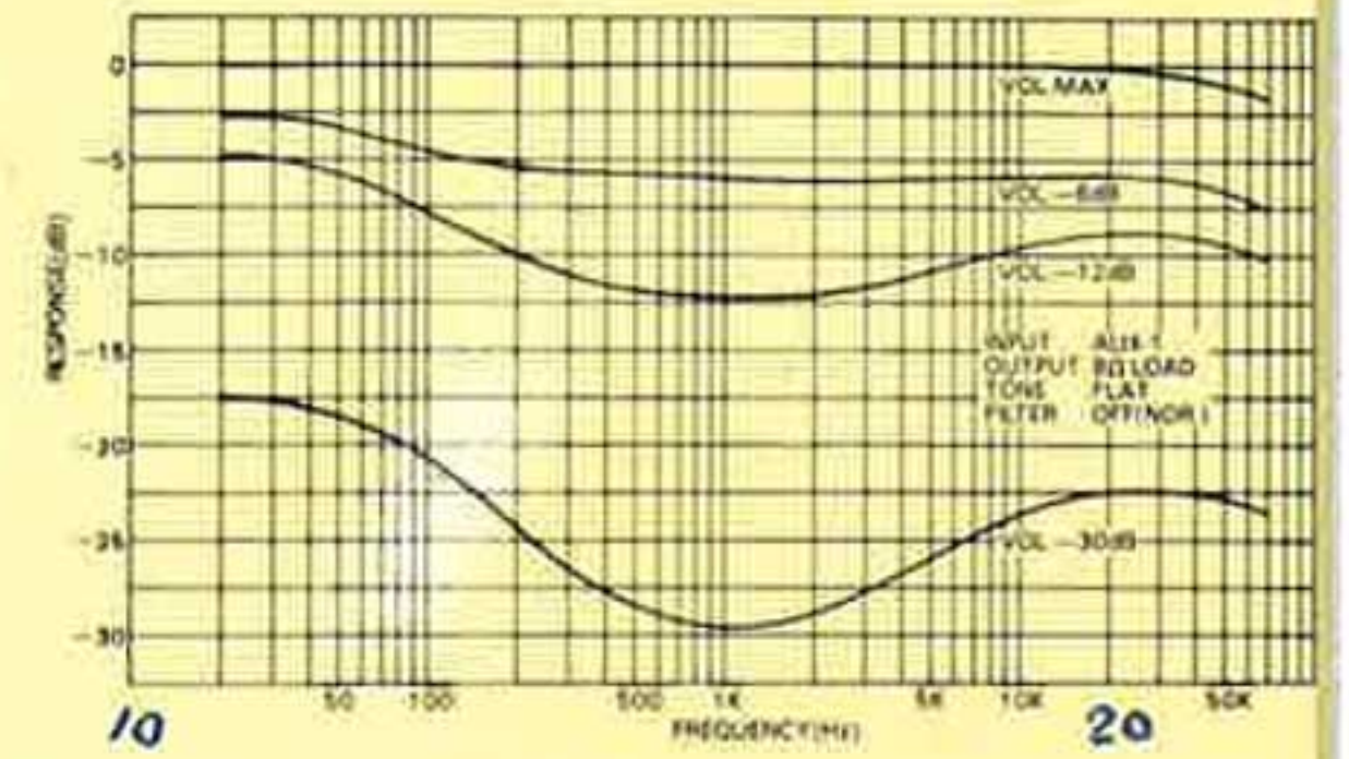
LOUDNESS/LOW BOOST
