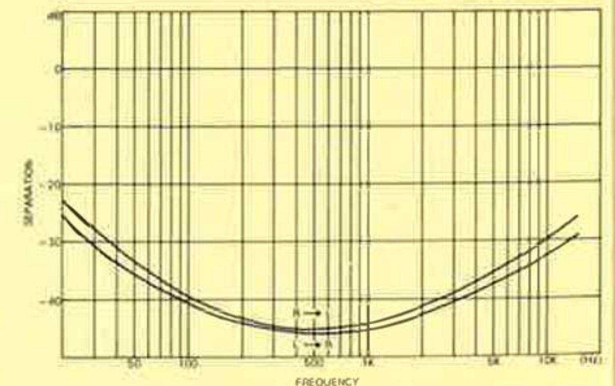
STEREO SEPARATION
