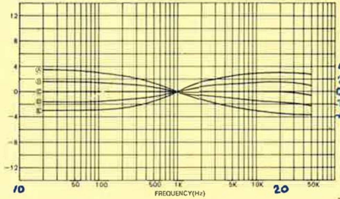
FILTER
