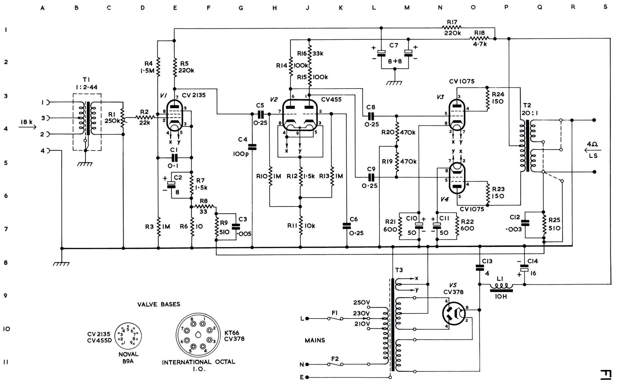
LOUDSPEAKER AMPLIFIER LSM/10 CIRCUIT SERIAL Nos 101 TO 470
