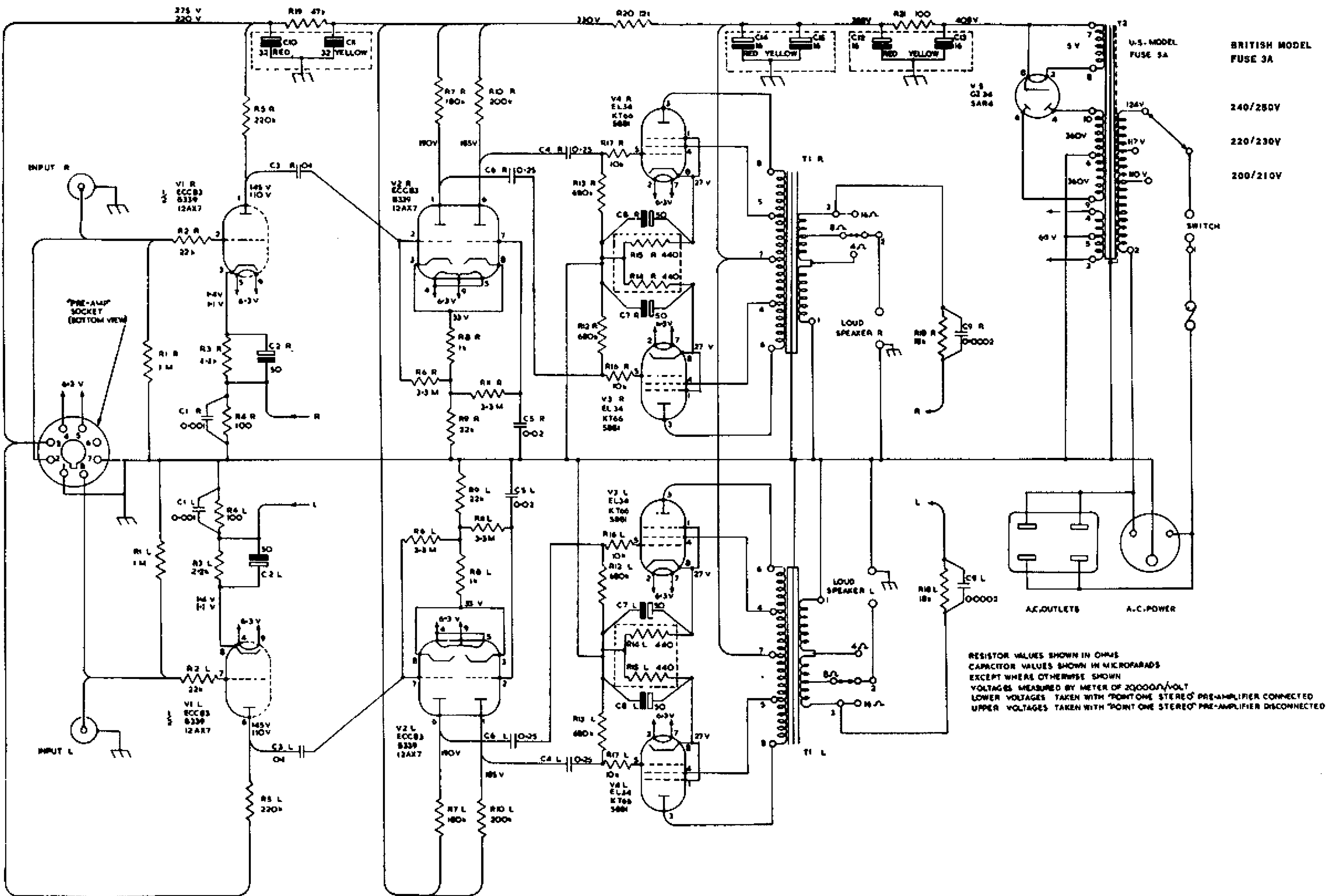
CIRCUIT DIAGRAM
