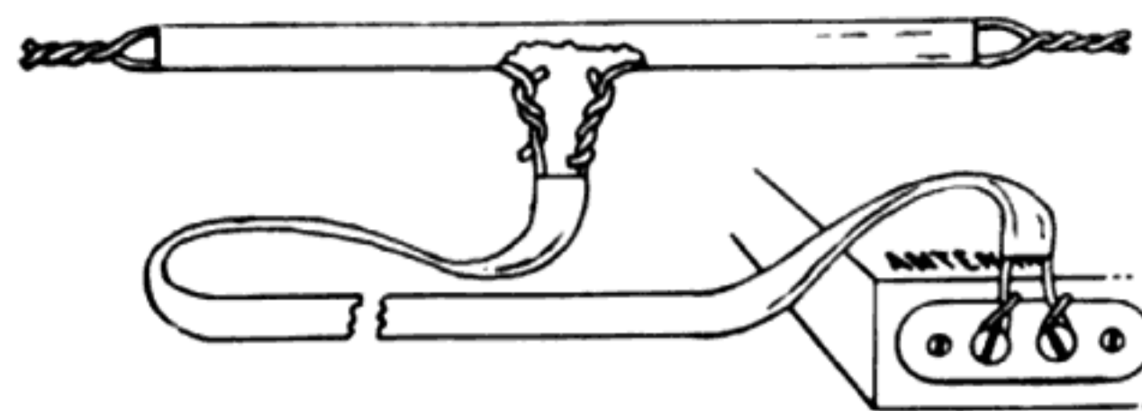
CONNECTION OF FOLDED DIPOLE ANTENNA
