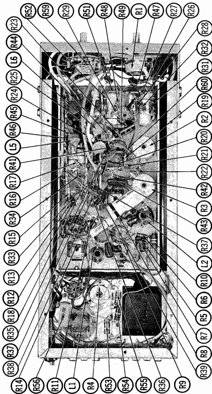
CHASSIS BOTTOM VIEW - RESISTOR & INDUCTOR IDENT.
