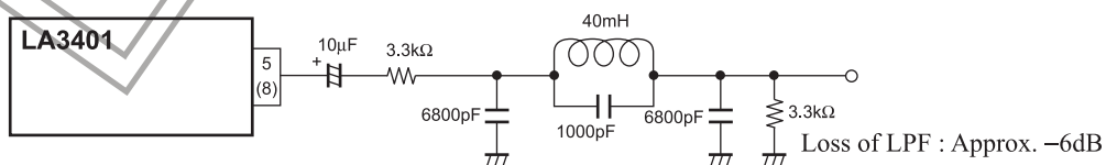
Fig. 16 Sample LC filter circuit (including de-emphasis circuit)
