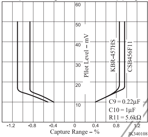
Capture Range Characteristic (4) Fig. 4
