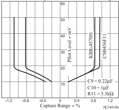
Capture Range Characteristic (2) Fig. 2
