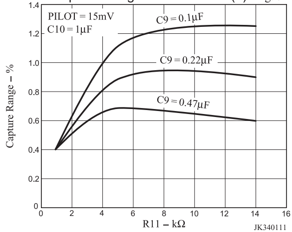
Capture Range Characteristic (5) Fig. 5
