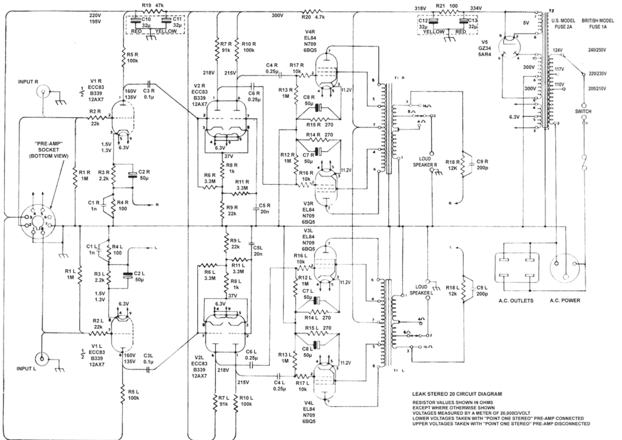
Leak Stereo 20: circuit for 3921 output transformers
