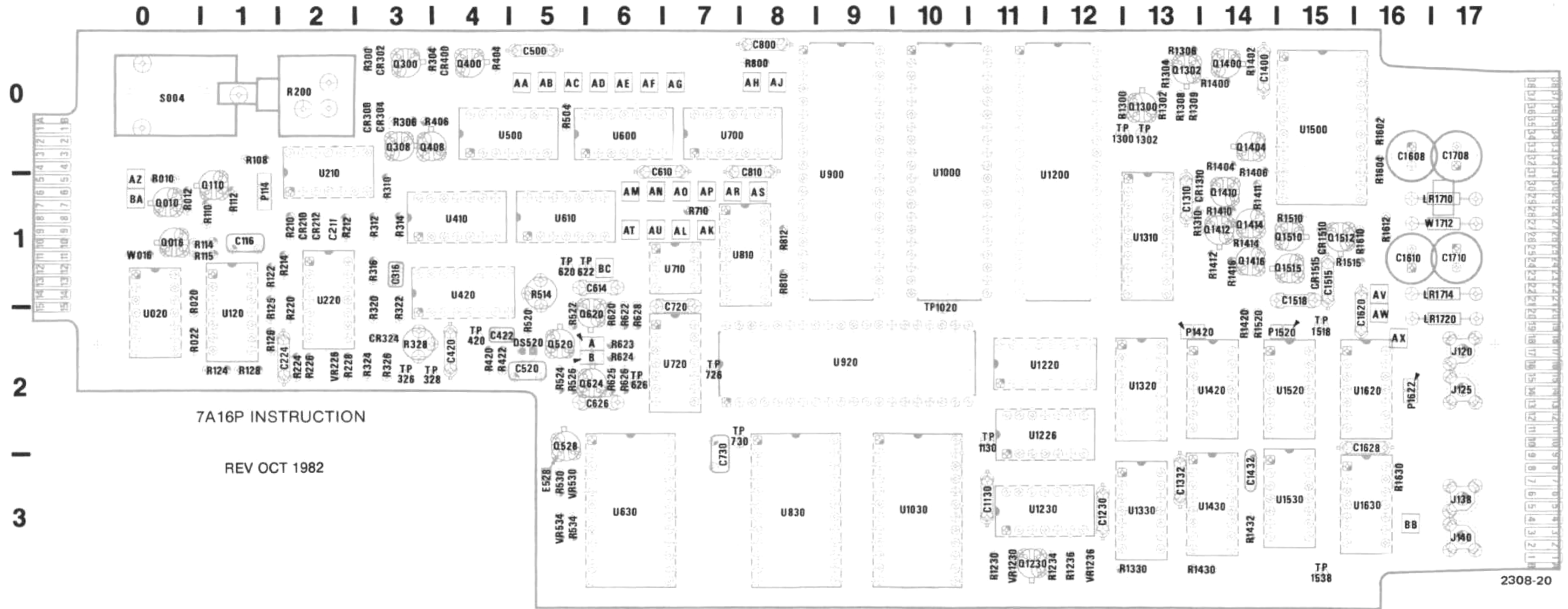
Fig. 8-7. A30 Programming Logic Board.
