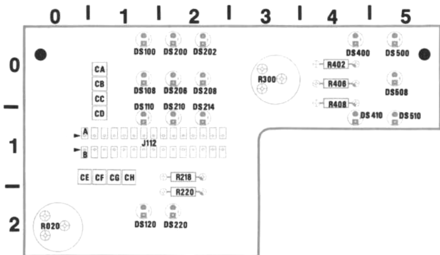
Fig. 8-8. A50 Switch Board.
