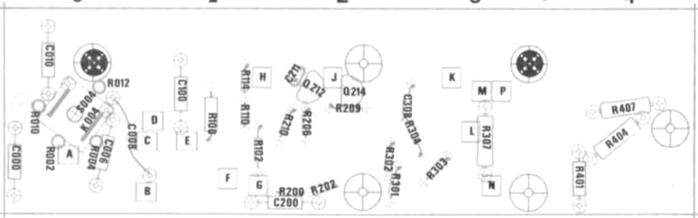
Fig. 8-1b. A10 Attenuator Board-Rear
