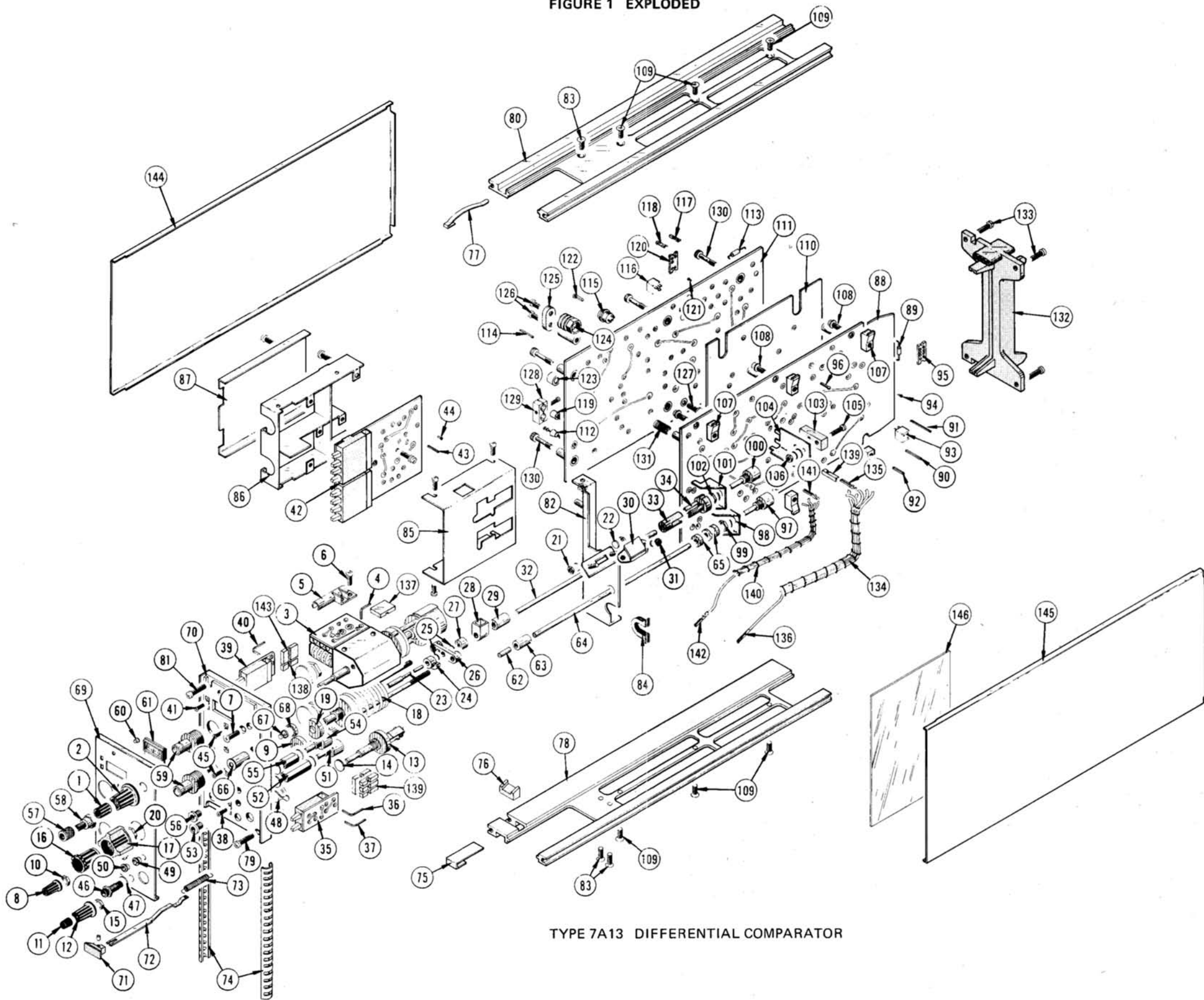
FIGURE 1 EXPLODED
