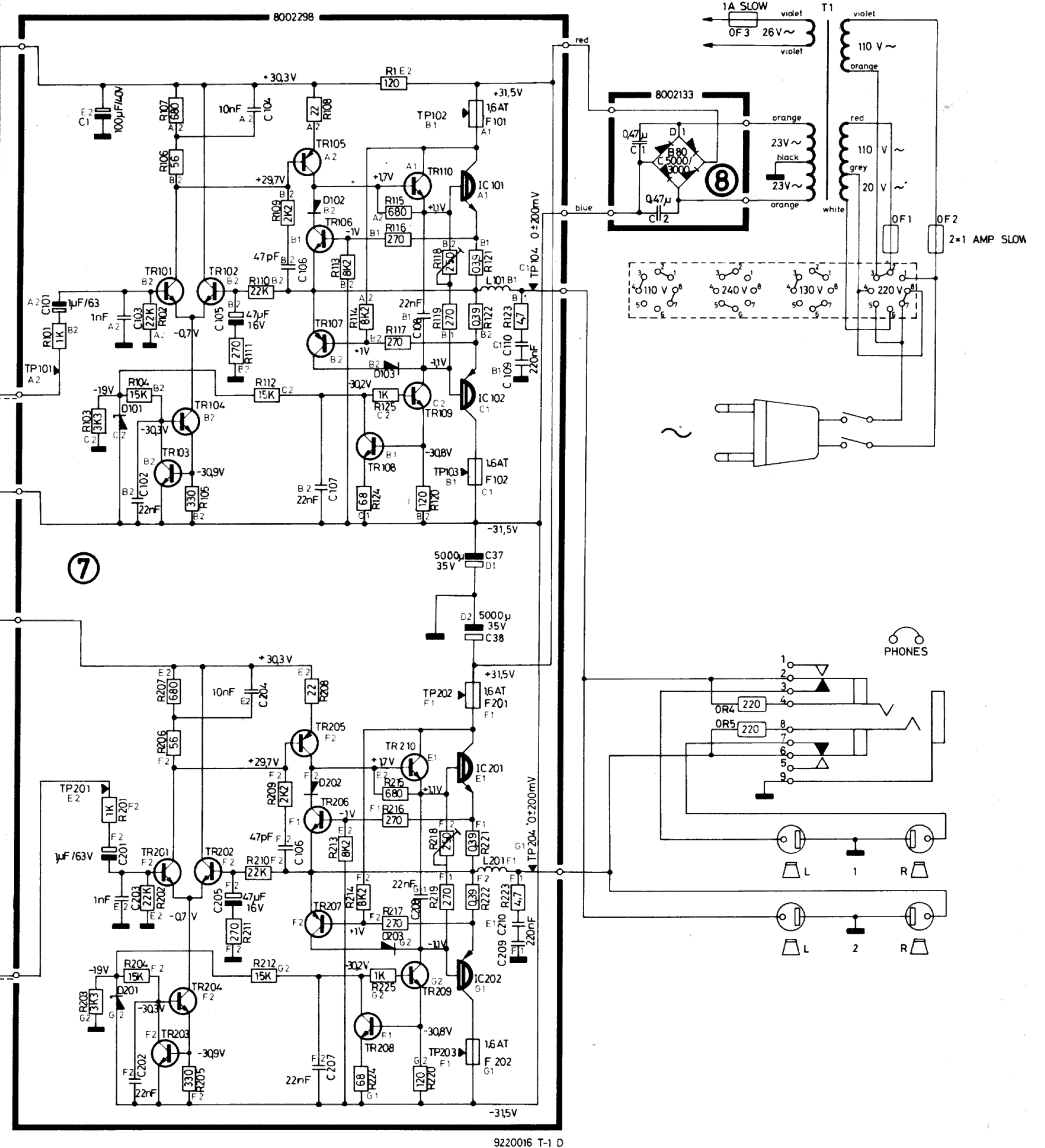
DIAGRAM TIL BEOMASTER 2000, TYPE 2801, FRA NR: 143001 DIAGRAM FOR BEOMASTER 2000, TYPE 2801, AS FROM NO: 143001 DIAGRAM FÜR BEOMASTER 2000, TYP 2801, AB NR: 143001
